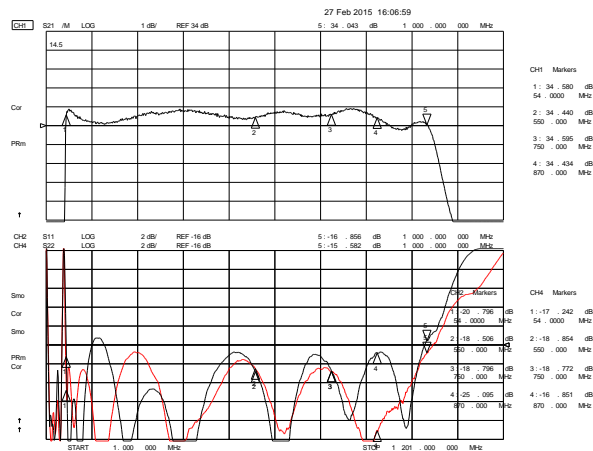
Fig. 1: B67C 2-PAC-C-COR rev 3 in new 1 GHz housing
