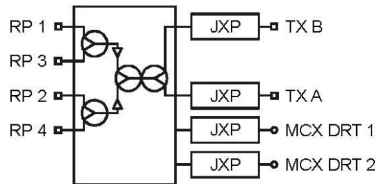
Single combined return, redundant option configuration block diagram
